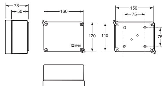
Caja ciega IP55 / Blind box IP55 - Ref. Item 3072
