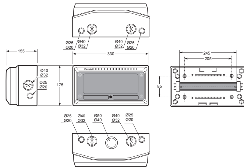
Caja Troquelada / Drilled box - Ref. Item 3964
